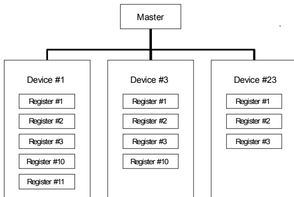
Illustration 1: Example Modbus™ Architecture
