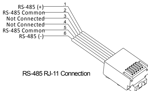
Illustration 2: Modbus™™ Cable Wiring
